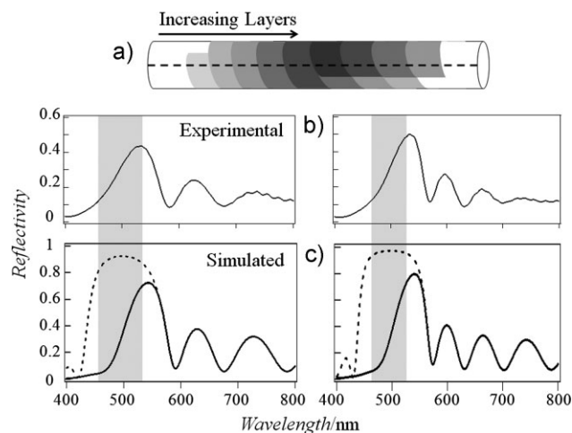
Figure 3. a) Helical roll-up was employed to enable access to different numbers of layers. Spectra were only taken along the dashed line. b) Experimental reflection spectra for six and eight layer points upon the polymer roll. Bragg stopbands are shown by the shaded areas. c) Simulated reflection spectra for six and eight flat bilayers of 160 nm PS and 10 nm Au. Rectangular stopbands arising from a purely dielectric multilayer stack are shown for an equivalent number of layers (dashed line).
